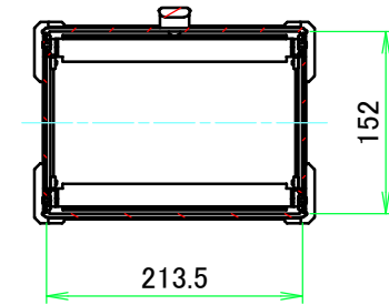
C-C (1:7)
