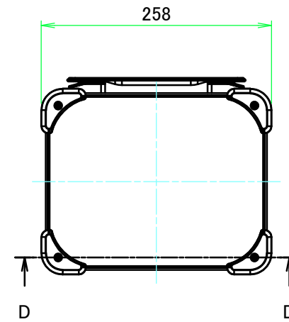
E view
