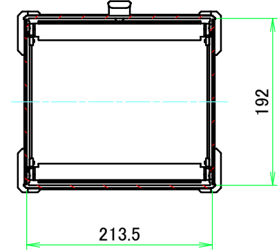
C-C (1:6)
