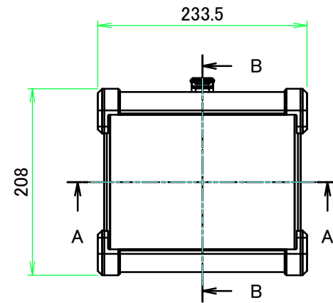
A view
