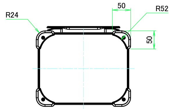
F view
