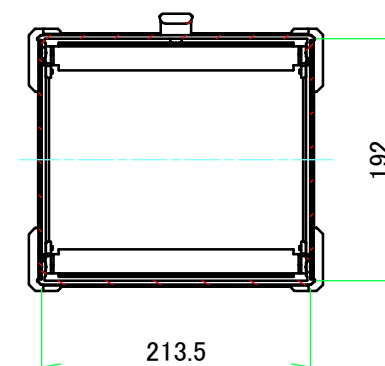
C-C (1:6)
