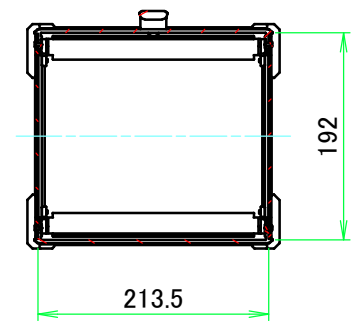
C-C (1:7)
