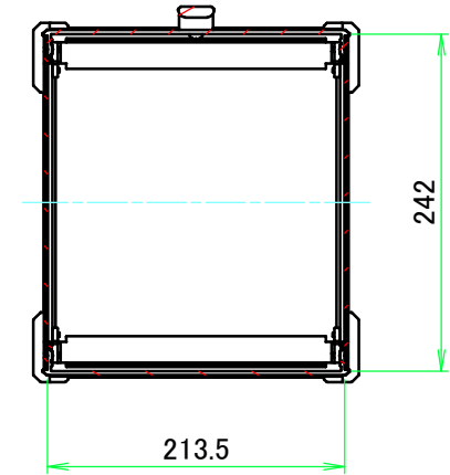
C-C (1:6)
