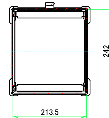
C-C (1:6.5)
