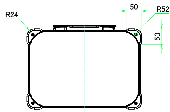
F view
