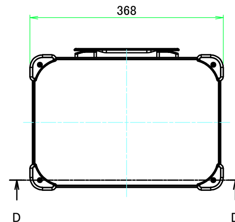
E view
