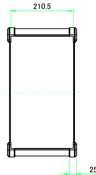
D view
