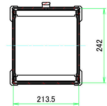
C-C (1:7.5)
