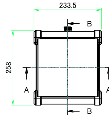
A view
