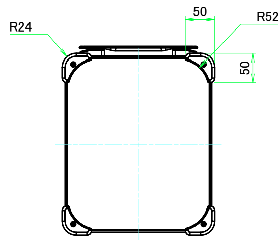
F view
