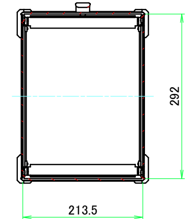
B view
