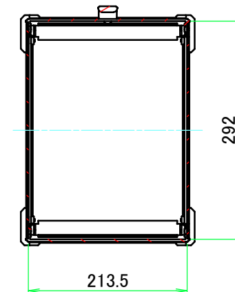
C-C (1:7)
