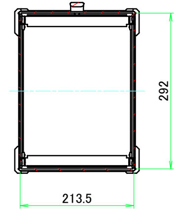
C-C (1:7)
