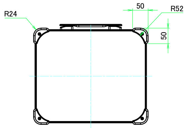
F view
