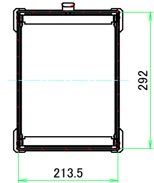
C-C (1:8)
