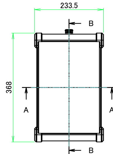
A view
