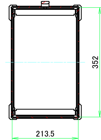
C-C (1:7.5)
