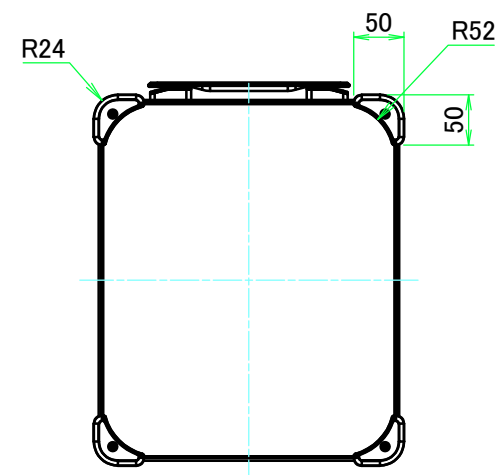
F view
