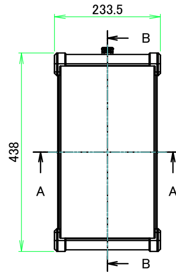
A view
