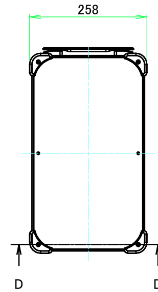
E view
