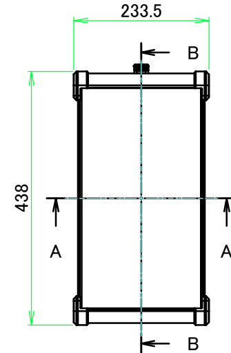
A view
