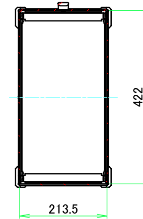
C-C (1:9)
