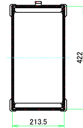
C-C (1:9)
