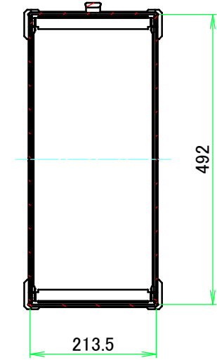
C-C (1:9)
