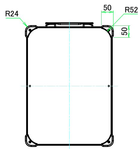
F view
