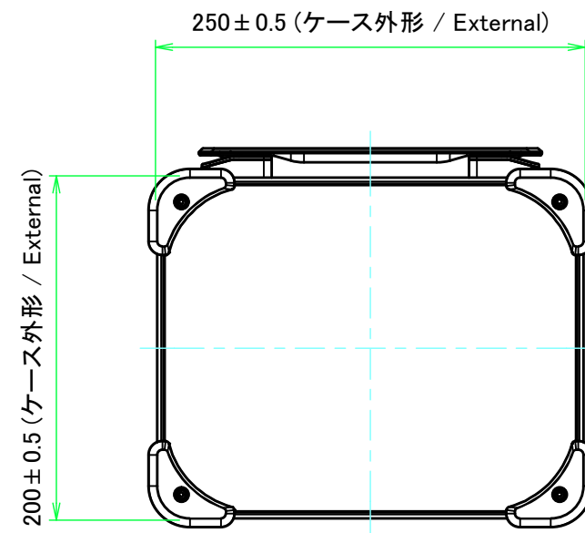
E view
