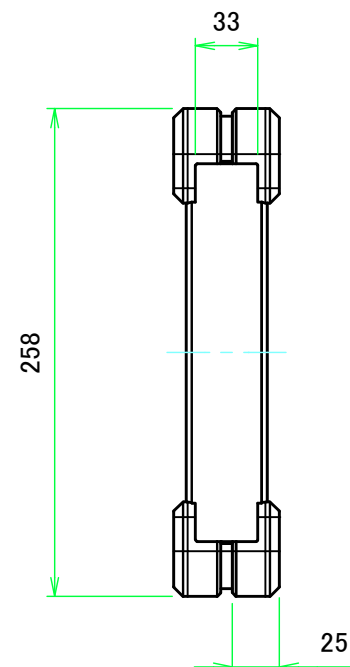
D view
