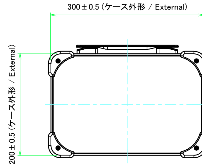
E view
