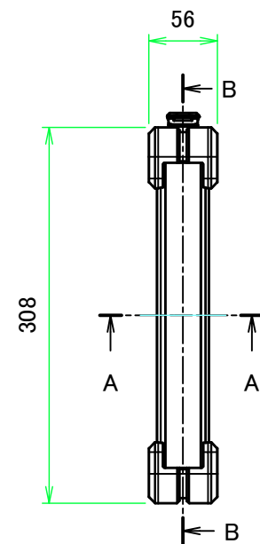
A view
