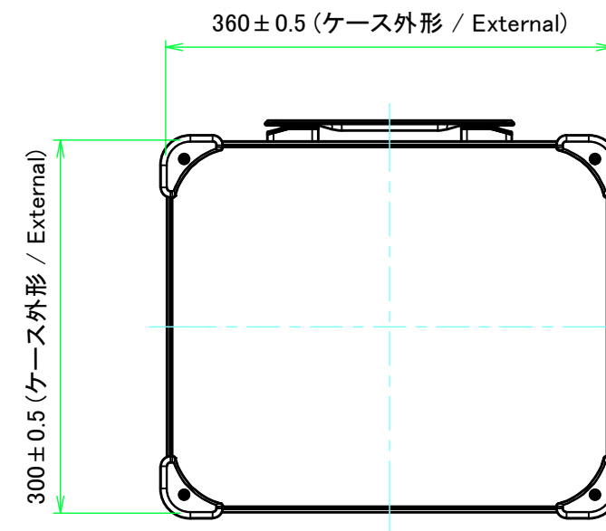
E view
