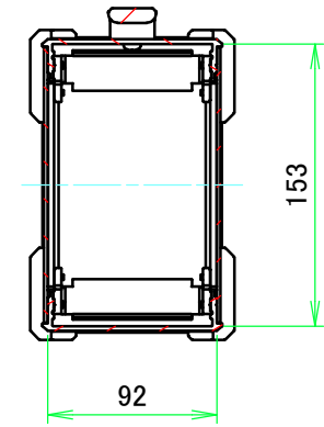
C-C (1:4.5)
