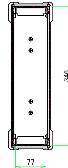
A-A (1:5.5)
