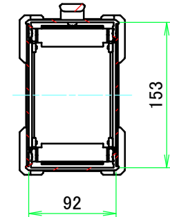
C-C (1:5.5)
