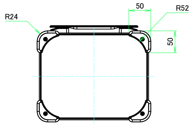
F view
