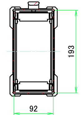
C-C (1:5.5)
