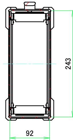
C-C (1:5)
