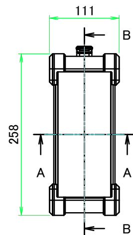
A view
