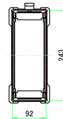
C-C (1:6)
