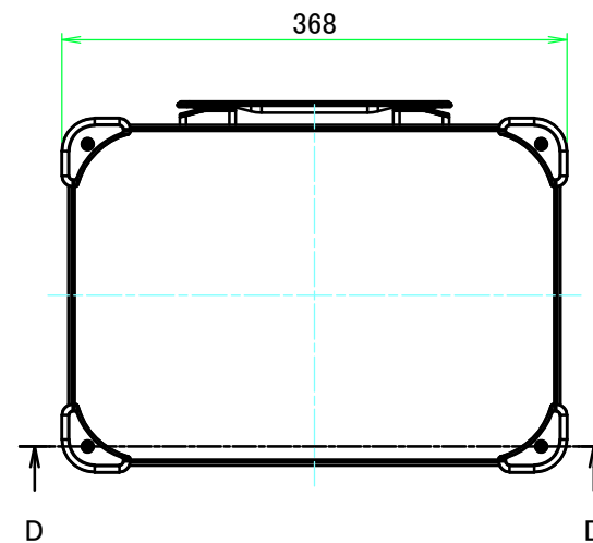
E view
