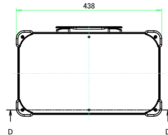
E view
