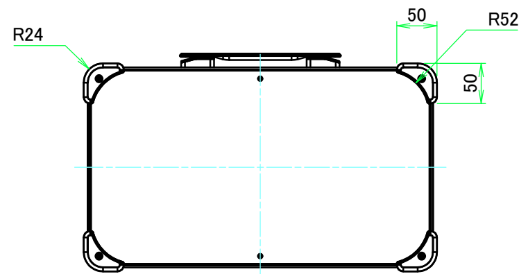
F view
