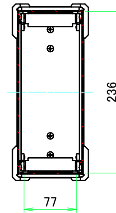
A-A (1:5.5)
