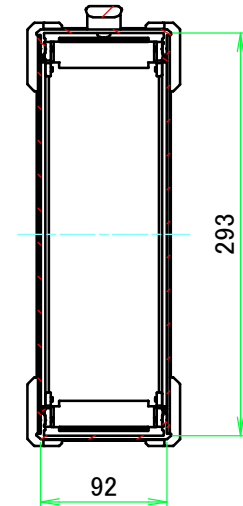
C-C (1:5.5)
