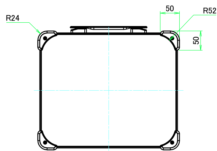
F view
