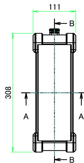
A view
