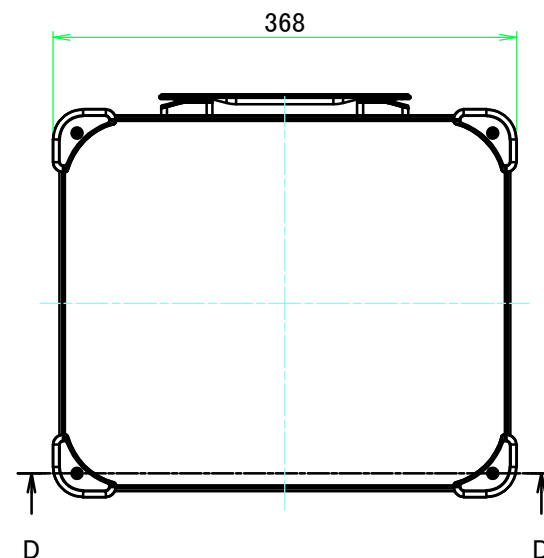
E view
