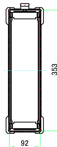
C-C (1:6.5)
