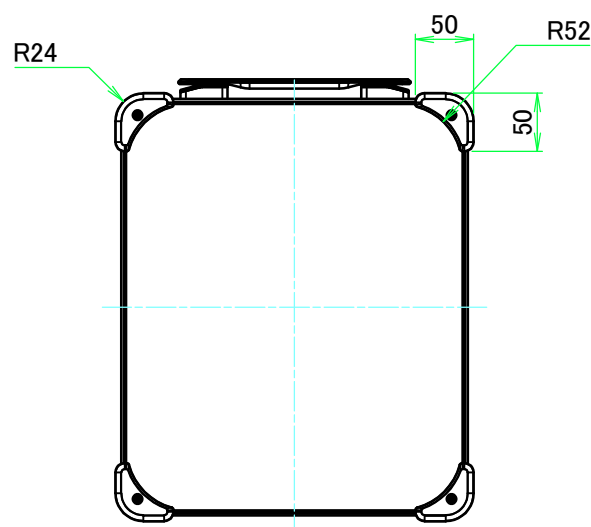
F view
