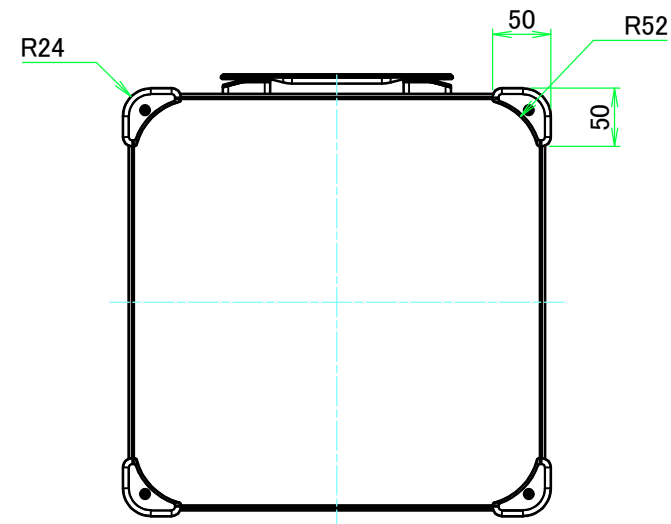
F view
