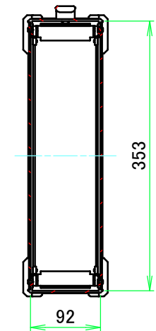
C-C (1:7)
