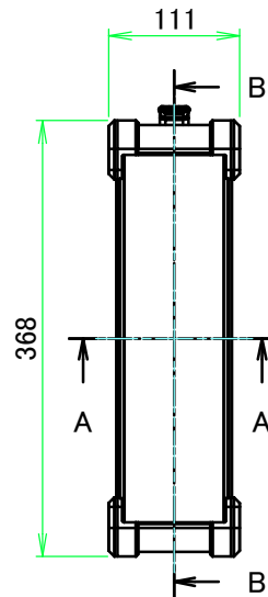
D view
