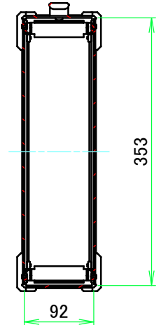
C-C (1:7)
