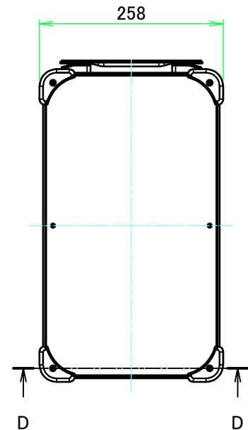
E view
