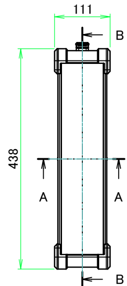
A view
