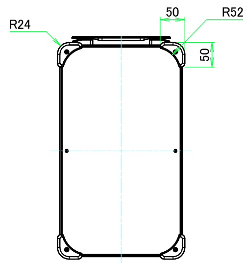
F view
