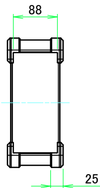
D view
