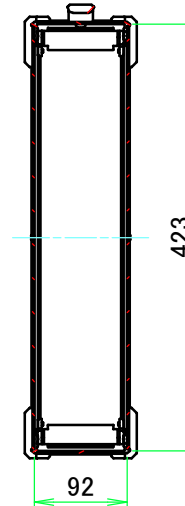
C-C (1:7.5)
