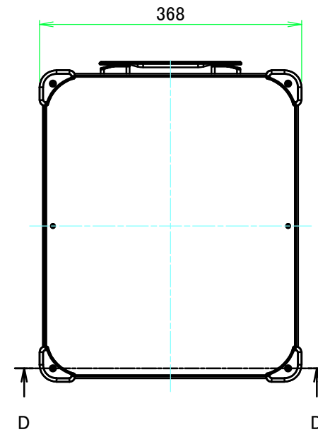
E view
