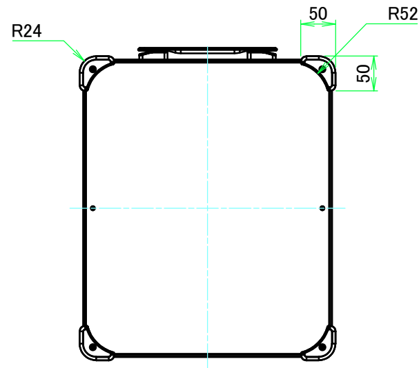
F view
