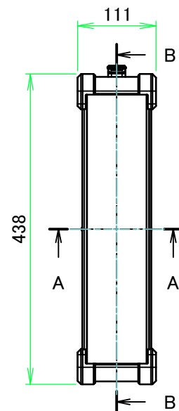
A view
