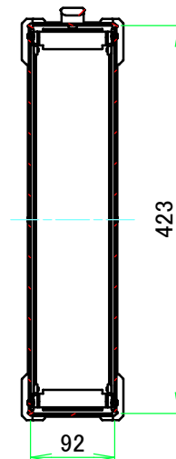
C-C (1:7.5)
