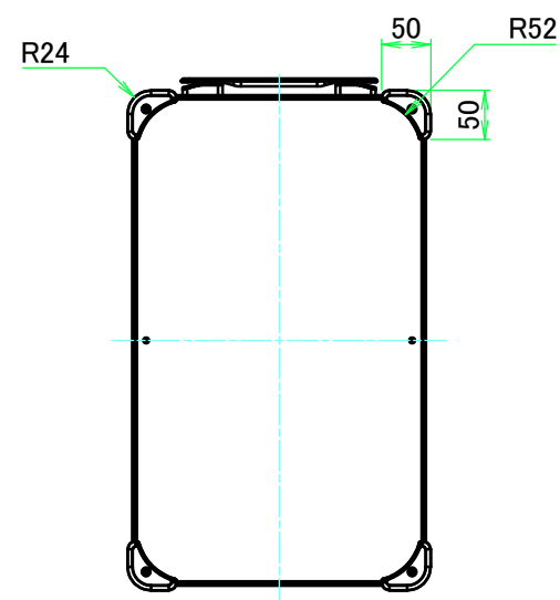
F view
