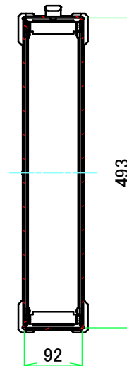
B view
