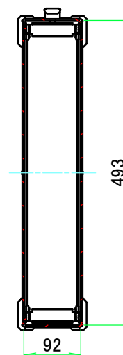
C-C (1:8.5)
