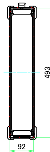
C-C (1:8.5)
