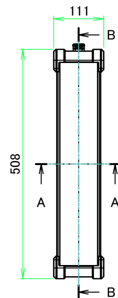
A view
