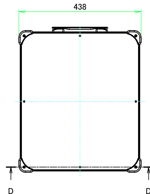
E view
