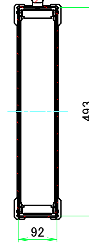
C-C (1:9)
