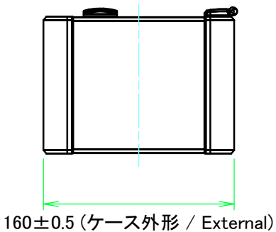
F view
