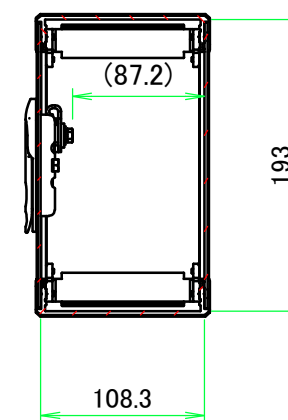
B-B (1:5)
