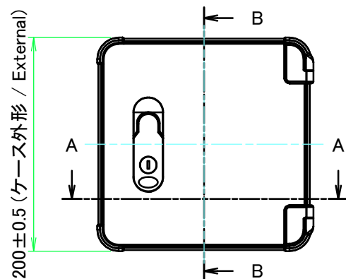
A view
