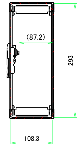
B-B (1:5)
