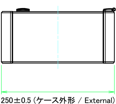
F view
