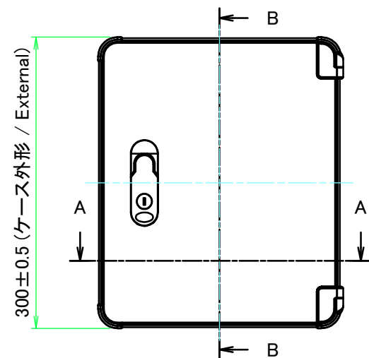
A view
