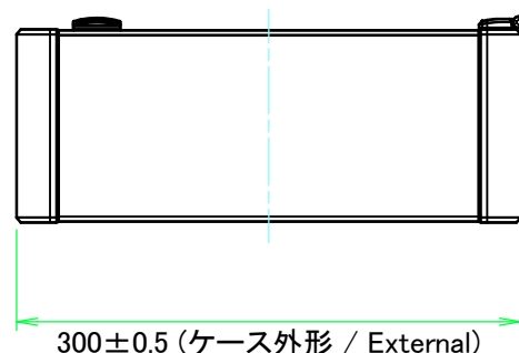
F view
