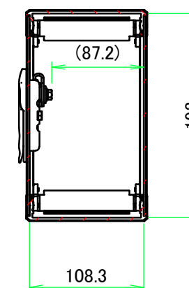
B-B (1:5)
