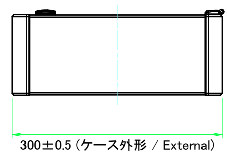
F view
