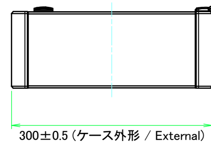
F view
